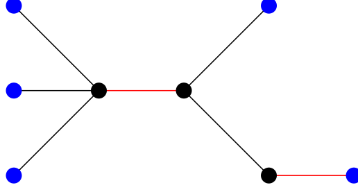
Fig. 2.1.3: The MST with contracted maximal paths (red edges). Leaves are blue, and internal vertices are black.
