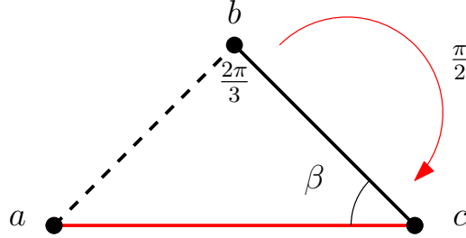
Fig. 2.2.3: Lemma 1: degree 2 case
