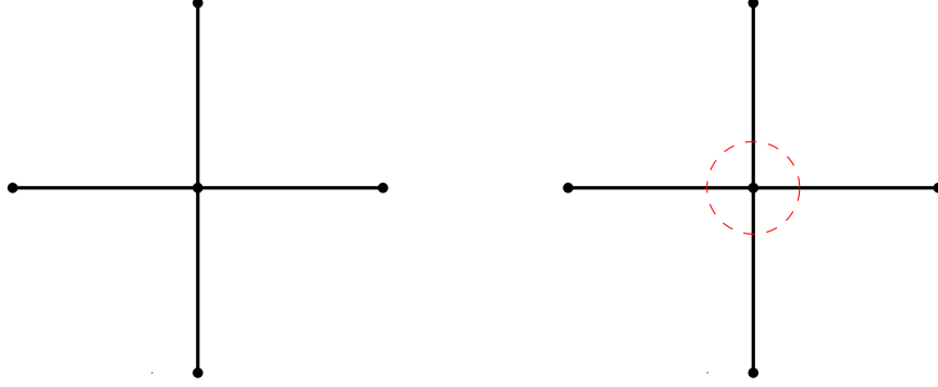
Fig. 1.2.5: Left: Euclidean MST, Right: Corresponding \bar{\pi/2} -MST
