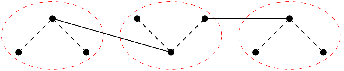
Fig. 1.2.3: A set of points in groups of 3 along the TSP tour. All points within a group are connected, and each group is connected. [2]
