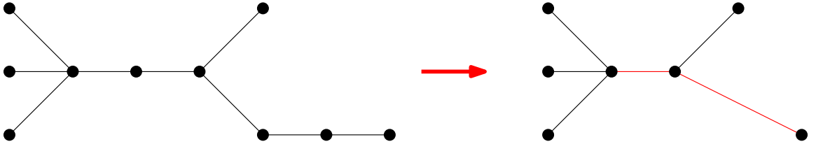
Fig. 2.1.2: The original MST (left) and MST with contracted maximal paths shown as red lines (right)
